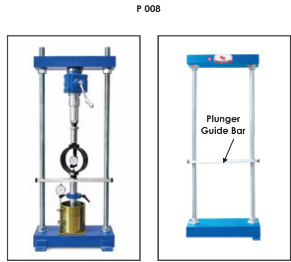
Lab test Set Up
